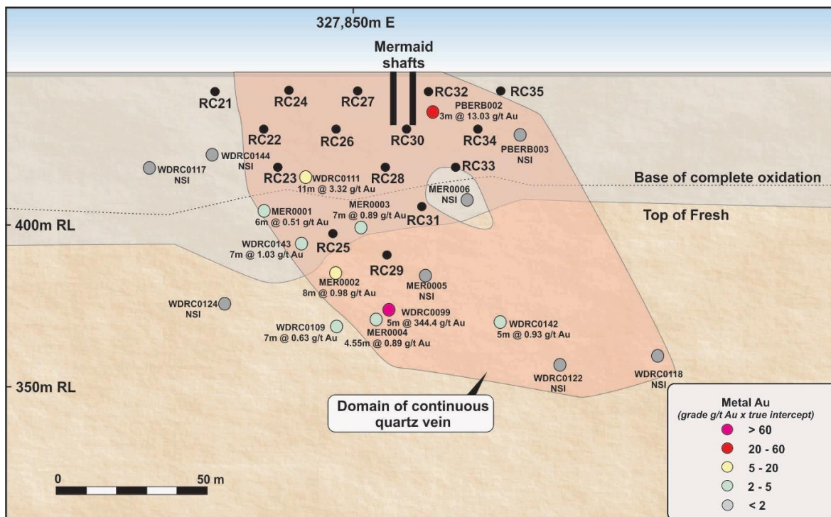
Figure 5 Long section of the Mermaid deposit showing pierce points of the November 2022 RC Drilling Programme
