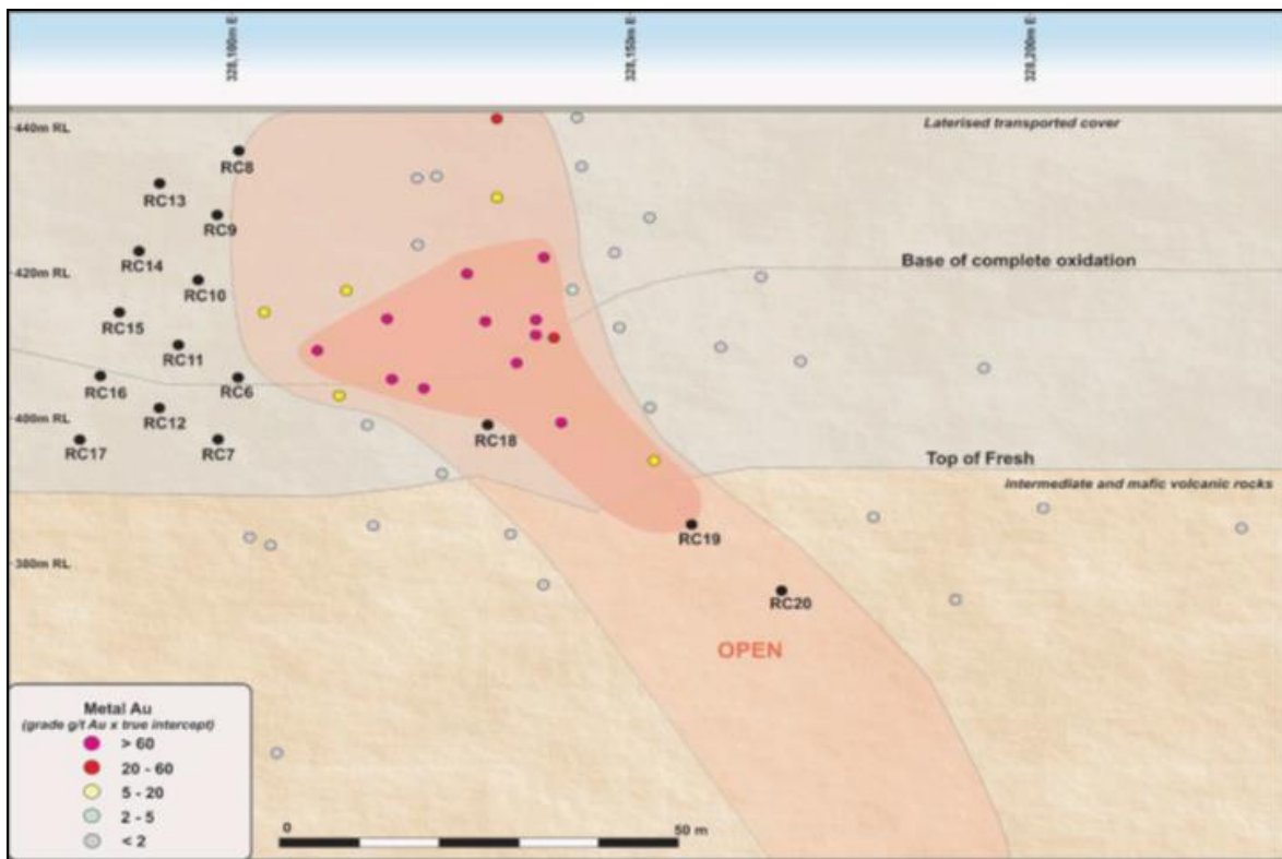
Figure 4 Long section of the Endeavour deposit showing pierce points of the November 2022 RC Drilling Programme
